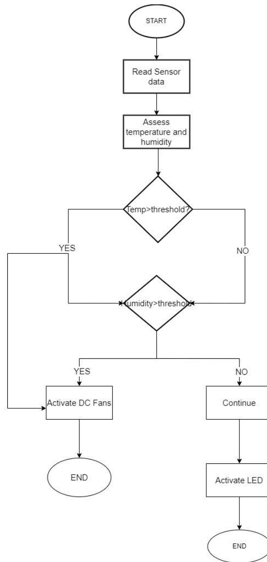
Figure 3: Flowchart 1.
