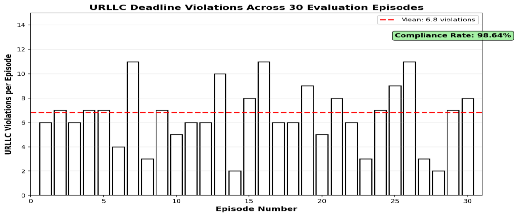
Figure 4.4: URLLC Deadline Violations Across 30 Evaluation Episodes
